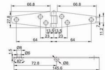
LIGHT STRAP HINGE Zinc Plated
